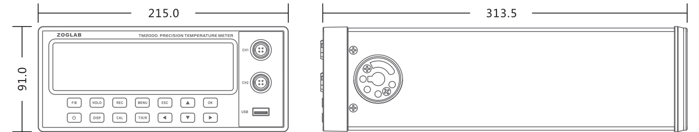
Dimensions(mm)
