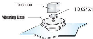
Fig. 3: Adhesive Mounting
