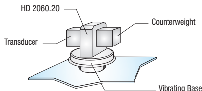
Fig. 5: Use of counterweights
