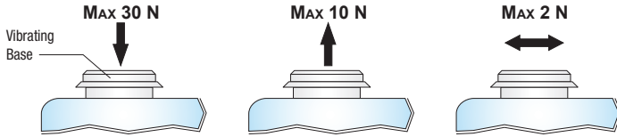
Fig. 2: maximum load limits for vibrating base
