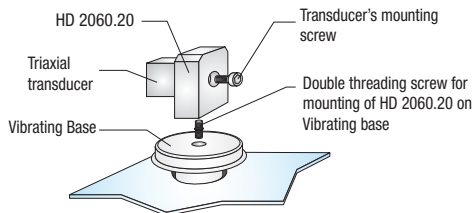
Fig. 4: Use of adapter HD 2060.20
